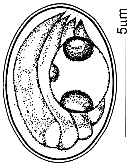
FIGURE 1. Sporulated oocyst of Cryptosporidium galli containing 3 granules within a spherical residual body surrounded by 4 banana-shaped sporozoites.
